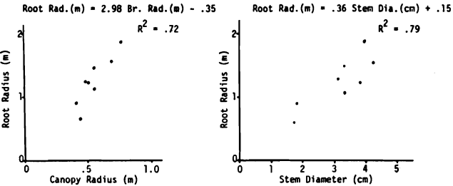
Fig. 2. Branch radius and stem diameter related to root radius. Each point represents data from one tree.
